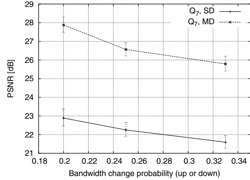
Fig. 5. Transmission quality for The Transporter base layer (QP=7) with different node mobilities modeled by the bandwidth change probability.
