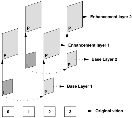
Fig. 2. Spatial scalable descriptor video coding with D = 2 temporal descriptors, which we also refer to as multiple descriptor (MD) encoding.
