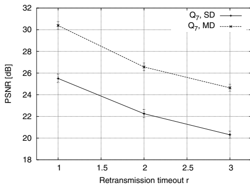
Fig. 4. Transmission quality for The Transporter base layer (QP=7) with different reconnection timeout durations.
