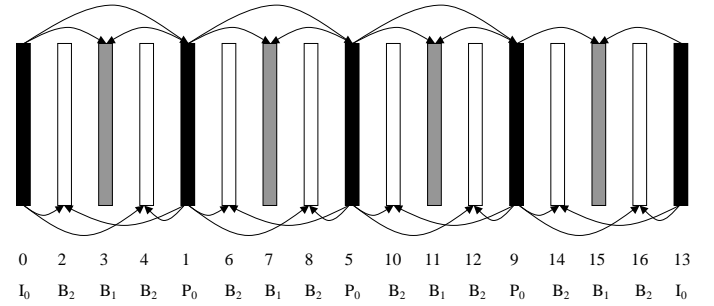
Fig. 1. Illustration of frame dependencies with classical B frames for an example with g = 16 frames in a GoP and b = 3 B frames between successive I and P frames. The frames are depicted in the display order. The encoding order is given by the top row of numbers, and the bottom row indicates the frame type in the display order.
