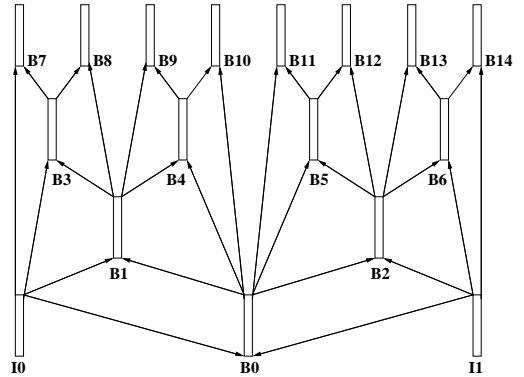
Fig. 2. Hierarchical B frames in encoding order with GoP structure with 15 B frames and no P frames.
